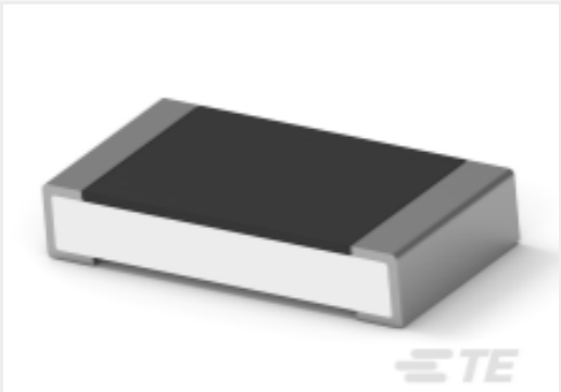
TE 产品编号5-2176391-8 RQ 1206 48K7 0.1% 10PPM 5K RL
