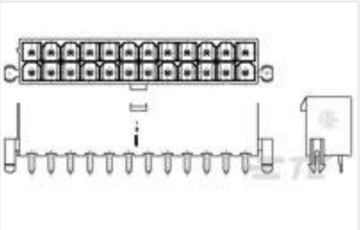
TE 产品编号1586039-4 4P VAL-U-LOK VRT HDR W/P V2
