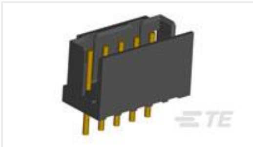
TE 产品编号292133-5 CT P/HDR ASSY BOX V 5P W/O KIN
