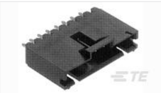
TE 产品编号5-103735-7 08 MTE HDR SRST LATCH .100CL
