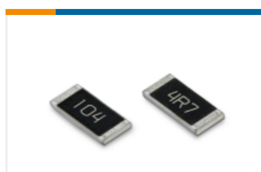
TE 产品编号3-2176456-5 CPF 0603 2R26 0.1% 25ppm 1K RL
