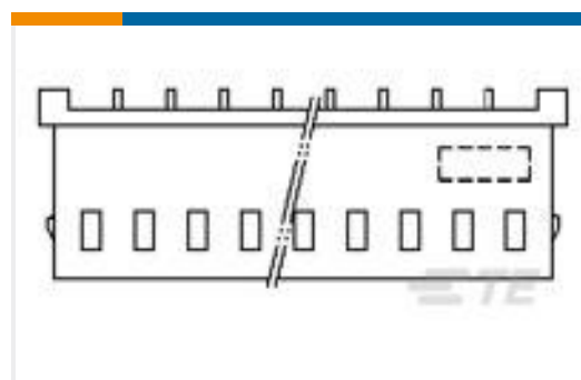
TE 产品编号1470222-2 HPI 2.5MM EMIX HOUSING 2P
