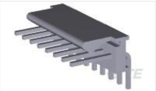
TE 产品编号640457-8 08P MTA100 HDR ASSY SQ R/A F/L
