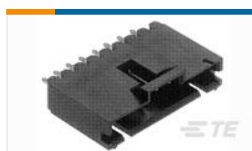
TE 产品编号5-103735-4 05 MTE HDR SRST LATCH .100CL
