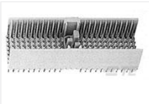
TE 产品编号352332-1 2MM HM TYPE A MALE HDR 154 POS
