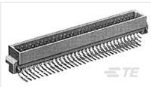
TE 产品编号5650907-5 ASSY,PIN,EUROCARD;TYPE C,LEAD-FREE,150 P
