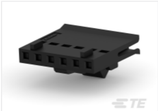
TE 产品编号 487526-5 006 HOUSING FFC RCPT 100CL SR
