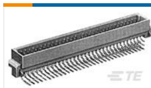
TE 产品编号650948-5 048 EURO TYPE C PIN ST ASSY
