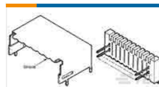
TE 产品编号5650922-5 ASSY,PIN,EUROCARD,TYPE R,LEAD-FREE,150 P
