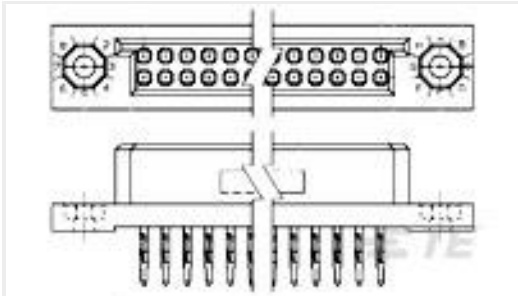
TE 产品编号5-533289-5 BOX II 2 ROW RECP ASSY 60 POS
