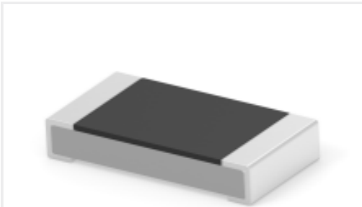
TE 产品编号3-2176392-4 RQ 1206 294K 0.1% 10PPM 5K RL
