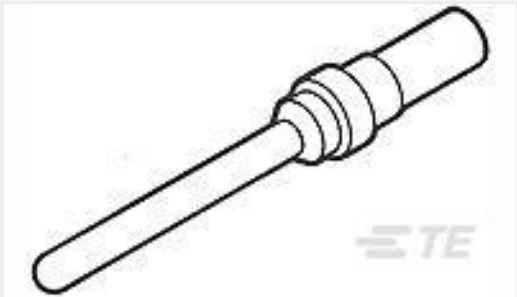
TE 产品编号1218266-1 CONT,CRIMP PIN,18AWG,109,SZ 20
