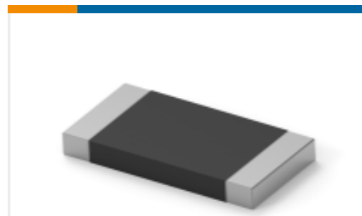
TE 产品编号2-2176422-5 TLRP 2512 3.0W R025 1% 25PPM 4K RL
