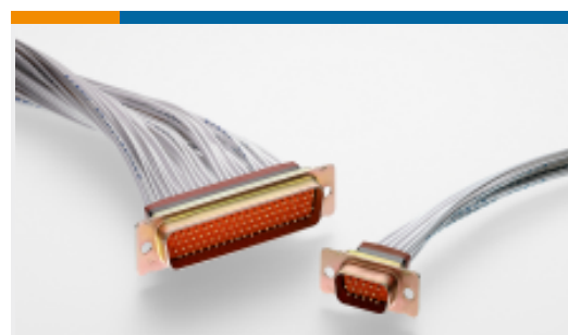
TE 产品编号2157480-1 AMPLIMITE IP67,SZ1, 109, 9 POS,IFS, PLUG
