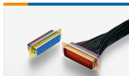
TE 产品编号1-2157480-3 AMPLIMITE IP67,SZ3, 109, 25 POS,IFS, PLUG
