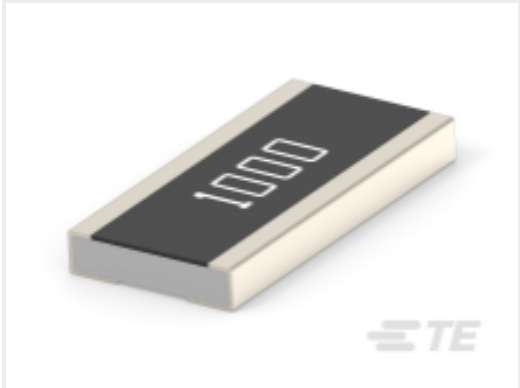
TE 产品编号1-2176563-2 3430 H2 1% 36K 100ppm 1k RL
