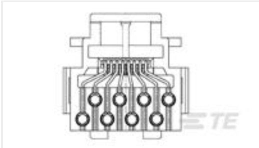
TE 产品编号216005-1 8P. TOOLLESS MOD J.
