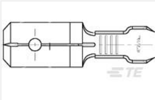
TE 产品编号42474-2 250 FASTON TAB 18-14 AWG TPBR
