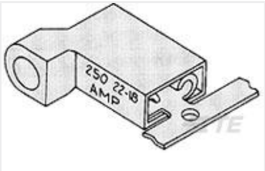
TE 产品编号9-520132-2 ULTRA-FAST 250 ASY FLAG REC 16-14 TPBR
