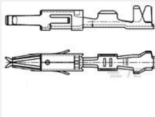
TE 产品编号962876-2 MT2 REC 1.6 Contact SWS Sn
