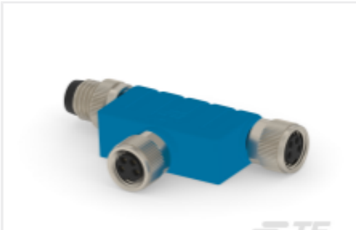
TE 产品编号T4082102004-000 M8 T DISTRIBUTOR MALE 4POS
