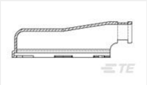
TE 产品编号66253-2 MALE CONTACT ASSY. (STRIP)
