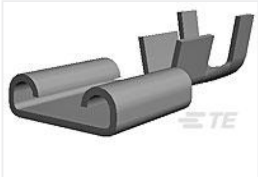
TE 产品编号170180-2 205 FASTON,REC.,18-14 AWG,TPBR
