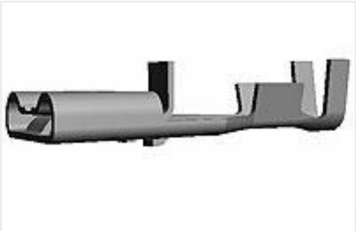
TE 产品编号170334-1 250 PL MIII,REC.,18-14 AWG,PTBR
