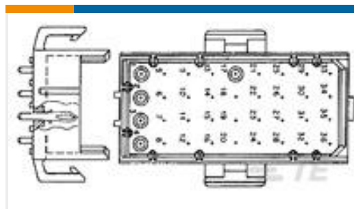
TE 产品编号640506-1 36P MR HDR ASSY V0
