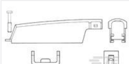
TE 产品编号1-552496-1 90 DEG COVER KIT-64 POS BLK
