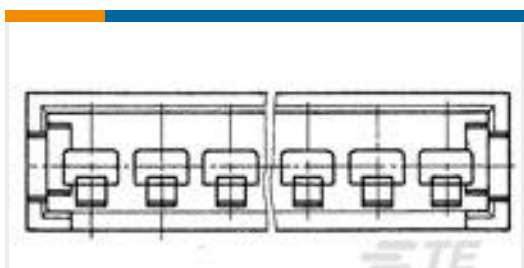
TE 零件编号1-86557-9 FFC,PIN CONTACT, ROUND WIRE,22-
