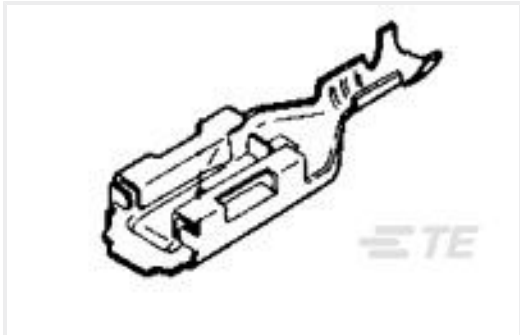
TE 产品编号170452-2 PL 250 AUTOMOTIVE REC 22-20 AWG PRE TPBR
