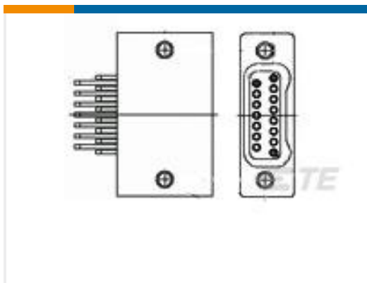
TE 产品编号9-1589483-9 STM009L2AN = SMT CONN
