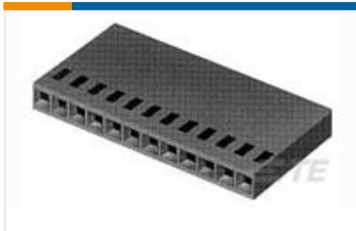
TE 产品编号87499-3 02 MODIV HSG SR MRKD .100CL
