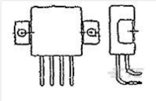
TE 产品编号2-1617752-5 FCA-210-HX2
