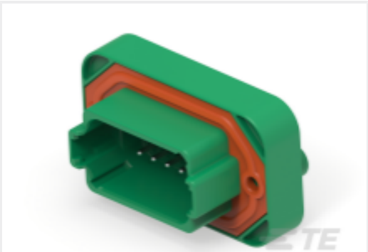
TE 产品编号DT15-12PC HDR, 12P, GRN, ST, NI/CU, C
