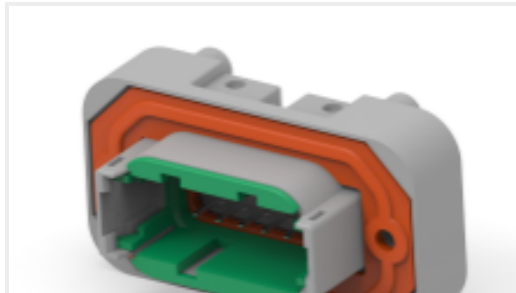
TE 产品编号DTM15-12PC HDR, 12P, GRY, ST, NI/CU, C
