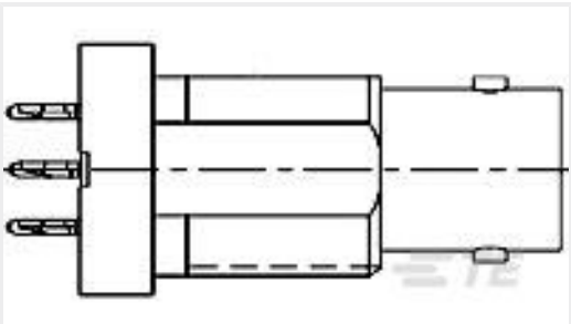
TE 产品编号5415456-1 JACK,PCB,PIN,BNC,75 OHM
