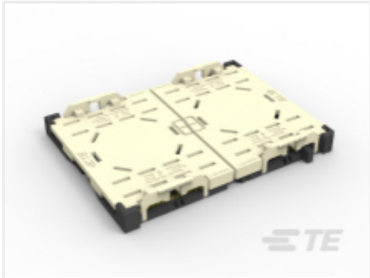
TE 产品编号1-2324271-2 LEFT SEGMENT LGA4189-4 SOCKET- P4 FOR ODM
