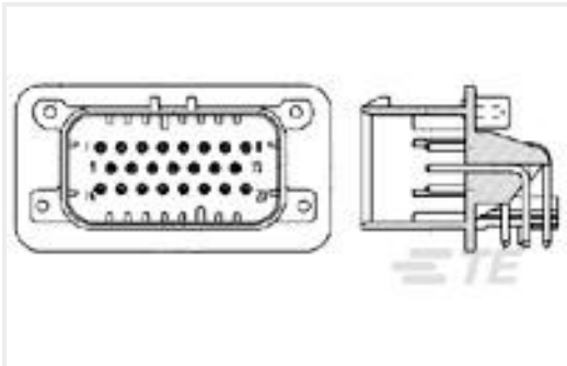
TE 产品编号1-770669-1 23POS, PIN DIA 1.3, HDR ASSY, 90DEG, COD 1
