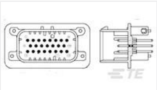
TE 产品编号1-776230-1 35POS,PIN DIA 1.3,HDR ASSY, 180DEG,COD 1
