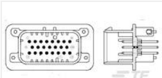
TE 产品编号776228-5 23POS,PIN DIA 1.3,HDR ASSY, 180DEG,COD 5
