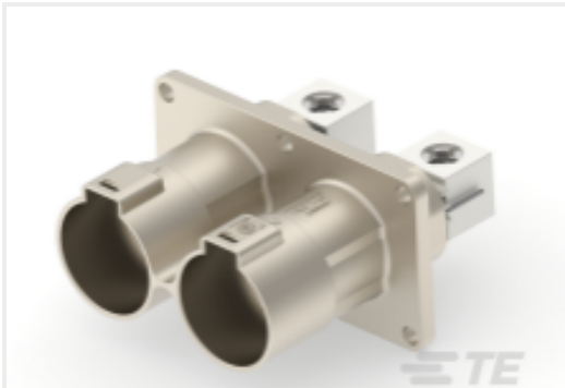
TE 产品编号1-2399607-1 2POS,HVP1400,ASSY,180DEG,COD A /B
