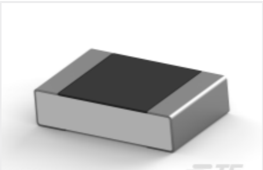
TE 产品编号5-2176380-4 RQ 0805 4K12 0.1% 10PPM 5K RL
