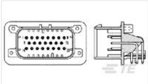
TE 产品编号770669-2 23POS,PIN DIA 1.3,HDR ASSY,90DEG, COD 2
