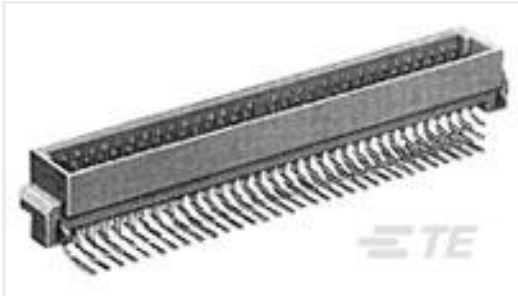
TE 产品编号5650913-5 ASSY,PIN,EUROCARD,TYPE C,LEAD-
