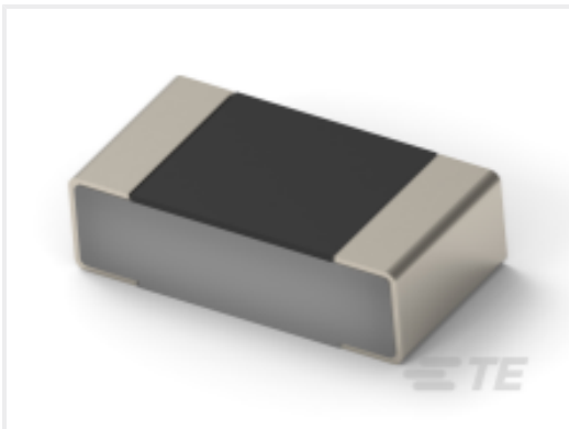
TE 产品编号2176467-4 TLRP 1206 1.0W R015 1% 50PPM 5K RL
