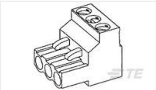
TE 产品编号796640-6 6 POS 5.0 MM R/A PLUG,TRM BLK
