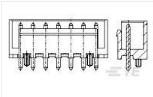
TE 产品编号1744357-4 3.96 EP SHROUDED HDR ASSY 4P W
