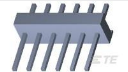
TE 产品编号640452-6 06P MTA100 HDR ASSY SQ STR
