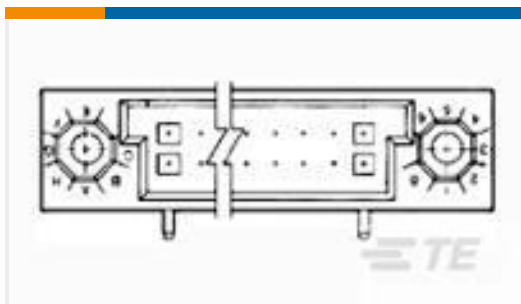
TE 产品编号532428-7 HDI RECP ASSY 2 ROW 80 POS
