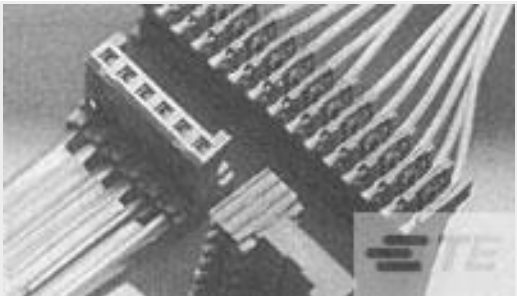
TE 产品编号144273-4 PLUG HE13 IDC 90 4 P AWG 24
