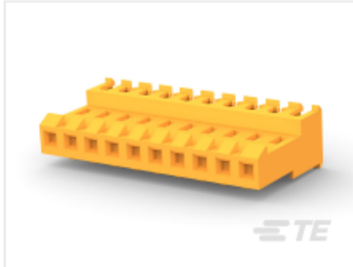
TE 产品编号 4-640599-0 10P MTA156 CONN ASSY 18AWG ORA
